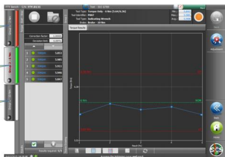
Automatic ISO6789
